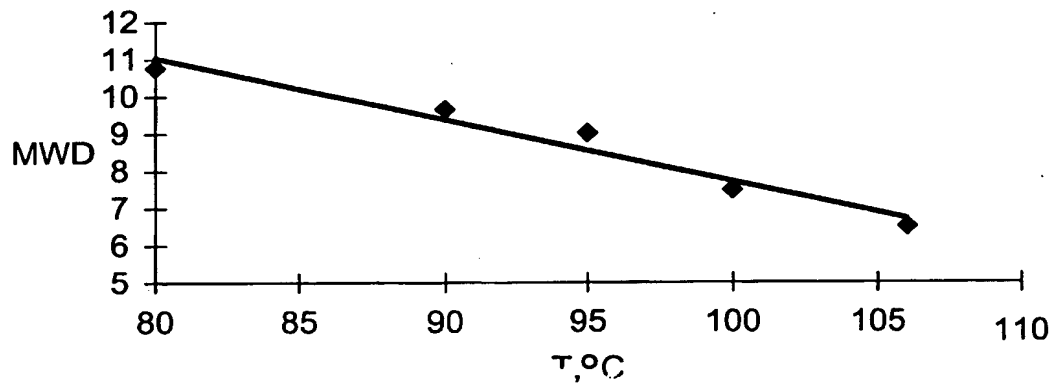
MWD by GPC vs T polymerisation
